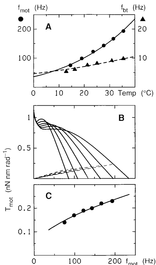
FIGURE 13 Dependence of motor frequency f_{\text{mot}} of freely swimming E. coli cells and body rotation frequency f_{\text{bt}} of tethered cells on temperature, as well as torque–frequency relations for counterclockwise rotation at different temperatures. (A) Data for f_{\text{mot}} (circles, left ordinate) and f_{\text{bt}} (triangles, right ordinate) are taken from Fig. 8 and Table 1 of Iwazawa et al. (1993), respectively; for both cases, \text{pH}_{\text{ex}} = 7 , hence \text{pH}_{\text{in}} = 7.43 and \Delta\psi_m = 125 mV (Fig. 4 A). The curves represent the result of the analysis based on the model. (B) Simulated torque–frequency relations (solid lines) at 14.5, 19.0, 23.5, 27.7, 31.5, and 35.5°C (from left to right along the abscissa) using the parameter values in Tables 1 and 2. The rate constant \alpha_{2,1} was calculated by means of Eqs. 42 and 43, and parameter fitting yielded the values for \Delta G_1^\#(T_{\text{ref}}) and \partial\Delta G_1^\#/\partial T listed in the second row of Table 3. Broken lines represent frictional drags at the temperatures mentioned above. They were calculated with values of the viscosity \eta of the medium approximated by that of water, and with k_{\text{mot}} = 1.67 \pm 0.03 pN·nm·rad -1 ·Hz -1 ·cP -1 (Eq. 39) obtained from parameter fitting. T_{\text{mot}} and f_{\text{mot}} at a given temperature are determined by the intersection of the corresponding solid and broken lines. They were used to construct the curves in (A) and (C). The circles in (C) represent data for T_{\text{mot}} taken from Table 1 of Iwazawa et al. (1993). The lines representing frictional drag for tethered cells are not shown in (B) for graphical reasons; parameter fitting yielded k_{\text{bt}} = 127 \pm 6 pN·nm·rad -1 ·Hz -1 ·cP -1 .
