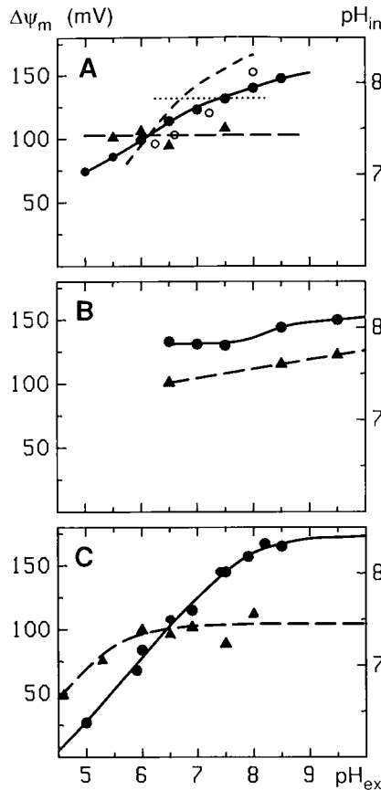
FIGURE 4 Dependence of membrane potential, \Delta\psi_m , and pH in the cytoplasm, \text{pH}_{\text{in}} , on pH in the suspending medium, \text{pH}_{\text{ex}} , for different species. Experimental data for \Delta\psi_m and \text{pH}_{\text{in}} are represented by closed circles and triangles, respectively. The solid and long broken lines were drawn through the points and served to determine values for the simulations. (A) E. coli at room temperature (closed symbols, data taken from Felle et al., 1980); short broken line, \Delta\psi_m at 30°C (Hirota et al., 1981); open circles and dotted line, \Delta\psi_m and \text{pH}_{\text{in}} at 28°C (Kashket, 1982). (B) Streptococcus at room temperature, data taken from Khan et al. (1990). (C) B. subtilis at 30°C, data taken from Shioi et al. (1980).
