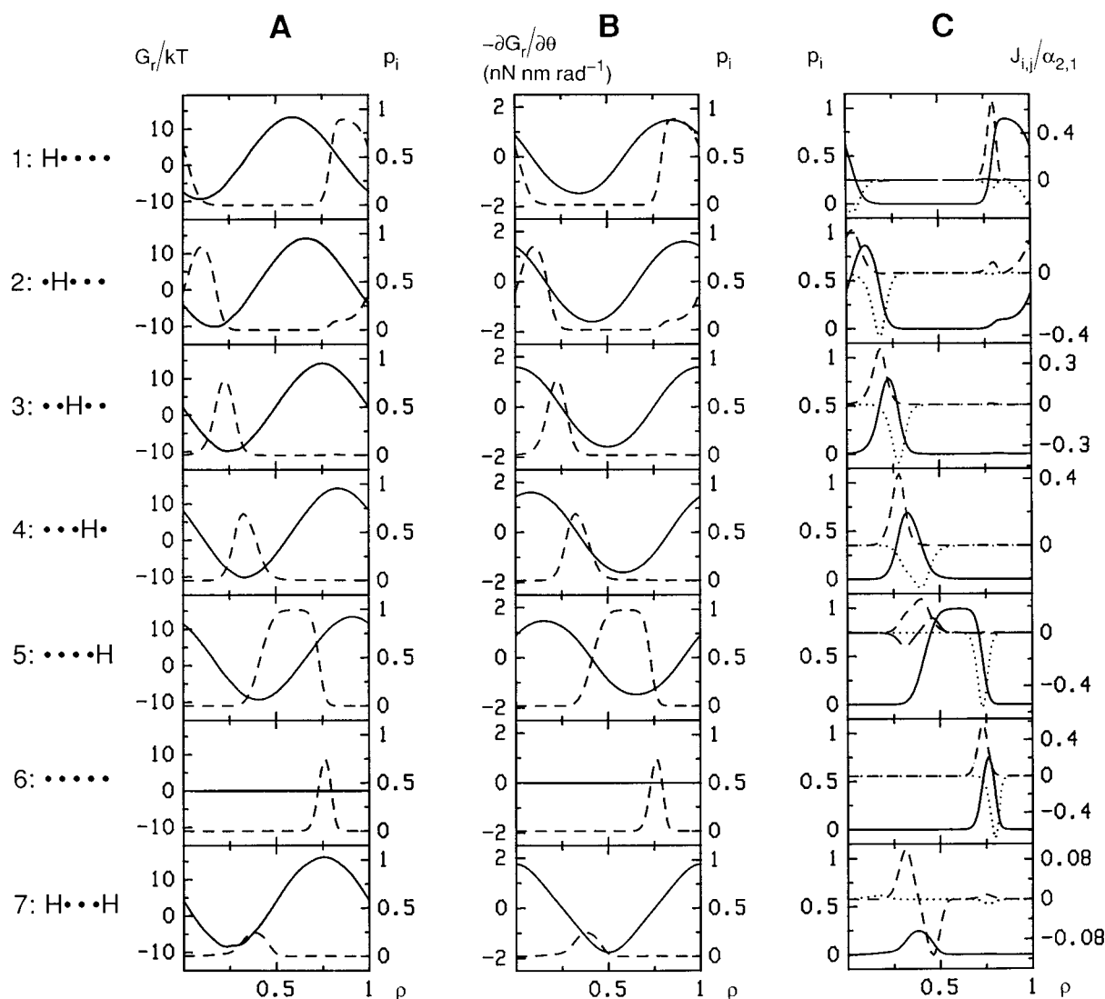
FIGURE 17 Free energy G_i of the states (A) and its partial derivative -\partial G_i/\partial\theta (B), as well as flows J_{i,j} between states (C) and probabilities p_i of states (A–C) at a given frequency, all as a function of rotation angle. The sequence of panels in a column from top to bottom corresponds to the numbering of states, as shown on the left (dots and H indicate empty binding sites and bound protons in a channel, respectively). The rotation angle is expressed by \rho (Eq. 5). G_i and \partial G_i/\partial\theta were calculated from Eqs. 6 and 15, together with Eqs. A2–A4, using the parameter values in Tables 1 and 2. The flows J_{i,j} were calculated from Eqs. 17 and 27–31, and with probabilities p_i obtained from the simulations of the torque–frequency relations shown in Fig. 9, A and B. The chosen frequency f'_{\text{mot}} = 0.04 is about at the end of the plateau (see inset of Fig. 18 A) and corresponds to f_{\text{mot}} = 100 and 190 Hz in Fig. 9, A and B, respectively. In (A) and (B), solid lines and left ordinates pertain to G_i/kT and -\partial G_i/\partial\theta , respectively, whereas the broken lines and right ordinates pertain to p_i . In (C), the p_i (left ordinates) are represented by solid lines, whereas the normalized flows J_{i,j}/\alpha_{2,1} (right ordinates) are represented by broken or dotted lines and are taken to indicate here flow into state i (that is, into state i when positive and out of state i when negative). Furthermore, the short broken and dotted lines indicate, respectively, flows between state i and the preceding or following states in the sense of the rotations shown in Fig. 2 B. The long broken lines refer specifically to J_{5,7} in the case of state 5 and J_{1,7} in the case of state 1. Note that J_{1,7} is so small that it appears to be zero in the first panel of C.
