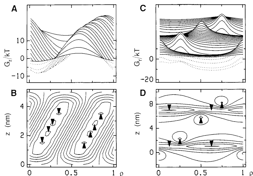
FIGURE 16 Free energy G_r due to electrostatic interaction between the charges on the rotor and a proton in a channel as a function of rotation angle and position z in the channel. ( A, B ) G_r was calculated from Eqs. 6 and A2–A4, using the parameter values in Tables 1 and 2, and is normalized by kT ; temperature 22.6°C. The G_r surface in ( A ) is viewed at an angle of 35°; top and bottom faces are indicated by solid and broken lines, respectively. The profiles pertain to different positions in the channel, which are spaced 0.25 nm apart, and the first profile is at the channel entrance on the periplasmic side, i.e., z = 0 (Fig. 1 A ). The rotation angle is expressed by \rho (Eq. 5). The contours in ( B ) indicate selected G_r/(kT) values between -12 and +12 with an increment of 2. ( C, D ) G_r/(kT) calculated as described by Elston and Oster (1997). Parameter values as given by the authors except for minor changes in the reciprocal electric screening distance ( 0.25 \text{ nm}^{-1} ) and the electric coupling strength ( 57.5 \text{ pN}\cdot\text{nm}^2 ). Presentation as in ( A ) and ( B ) except that the first profile in ( C ) pertains to z = -2 \text{ nm} and the values for the contours in ( D ) vary between -20 and +10 with an increment of 5. Upward and downward oriented arrow heads in ( B ) and ( D ) point at the positions of local maxima and minima, respectively.
