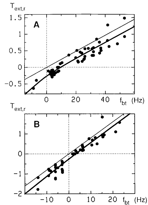
FIGURE 6 Minimal external torque necessary to synchronize cell and field rotation as a function of body rotation frequency f_{bt} . Tethered E. coli cells deficient in switching were exposed to a rotational electric field, and T_{ext,r} represents the minimal torque (in arbitrary units), which causes a synchronization of cell body and field rotation. Data points for (A) 9 small cells and (B) 11 large cells are taken from Fig. 5 of Iwazawa et al. (1993); temperature 25°C, pH_{ex} = 7 , hence pH_{in} = 7.43 and \Delta\psi_m = 125 mV (Fig. 4 A). The curves represent results of simulations with the model using the parameter values in Tables 1 and 2. The thin straight lines through the origin indicate the behavior of a fully broken motor. Parameter fitting yielded the following values: \alpha_{2,1} \times 10^{-5} s = 1.1 \pm 0.6 and 2.0 \pm 0.8 , k_{bt}/(nN \cdot nm \cdot rad^{-1} \cdot Hz^{-1}) = 0.099 \pm 0.010 and 0.33 \pm 0.03 for the data in (A) and (B), respectively. The same value for k_{ext} was used for both cases, and the fitting procedure then yielded 4.1 \pm 0.5 nN \cdot nm \cdot rad^{-1} .
