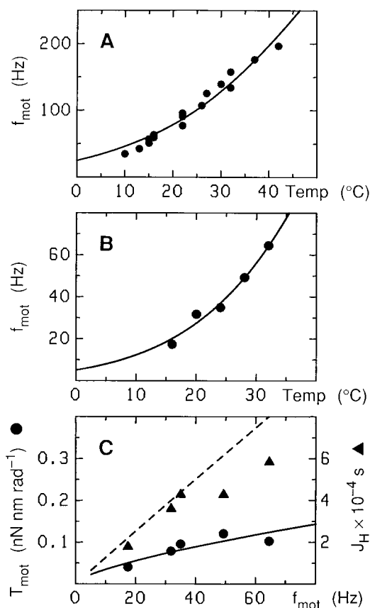
FIGURE 14 (A, B) Motor frequency f_{\text{mot}} of freely swimming Streptococcus cells as a function of temperature and (C) dependence of T_{\text{mot}} and J_H on f_{\text{mot}} at different temperatures. Data in (A) are taken from Fig. 4 of Lowe et al. (1987); \text{pH}_{\text{ex}} = 7.5 , hence \text{pH}_{\text{in}} = 7.5 and \Delta\psi_m = 132 mV (Fig. 4 B). Data in (B) and (C) are taken from Figs. 3 B and 4 B of Meister et al. (1987); \text{pH}_{\text{ex}} = 7.02 , \text{pH}_{\text{in}} = 7.62 , \Delta\psi_m = 45 mV (see legend to Fig. 11 B). The curves represent the results of analyses performed as outlined in the legend to Fig. 13. Values thereby obtained for \Delta G_1^\#(T_{\text{ref}}) and \partial\Delta G_1^\#/\partial T are listed in the third and fourth row of Table 3, whereas k_{\text{mot}}/(\text{pN}\cdot\text{nm}\cdot\text{rad}^{-1}\cdot\text{Hz}^{-1}\cdot\text{cP}^{-1}) = 4.3 \pm 0.2 and 2.5 \pm 0.2 , for the data in (A) and (B), respectively.
