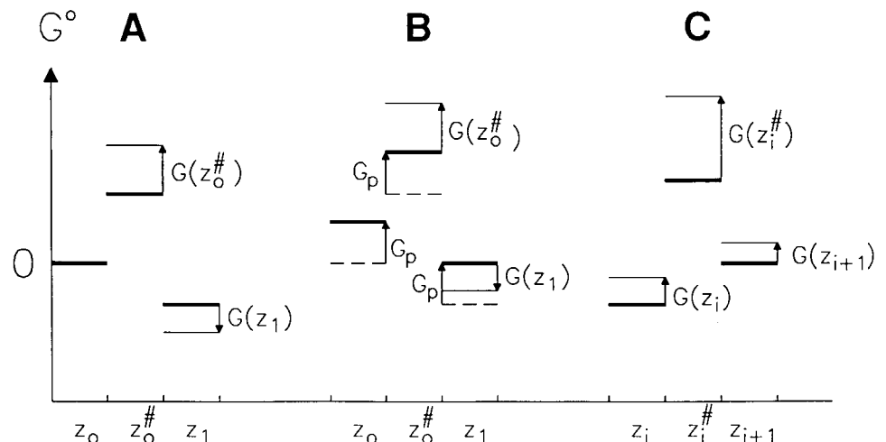
FIGURE B1 Hypothetical standard free energy levels governing proton transitions at a given value of \rho . (A) and (B) depict binding at the periplasmic entrance to a channel, (C) depicts a transition within the channel. The free energy levels before and after inclusion of electrostatic interactions due to rotor charges and protons in other channels (giving rise to the free energies G ) are represented by thick and thin lines, respectively. The effect of prior binding of a proton at the cytoplasmic end of the channel, which, due to electrostatic interaction, shifts the levels upward by a free energy G_p , is shown at (B).
